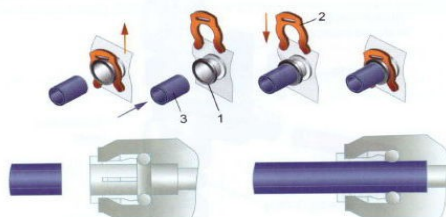
Figure 6. Connection of JG tubes
